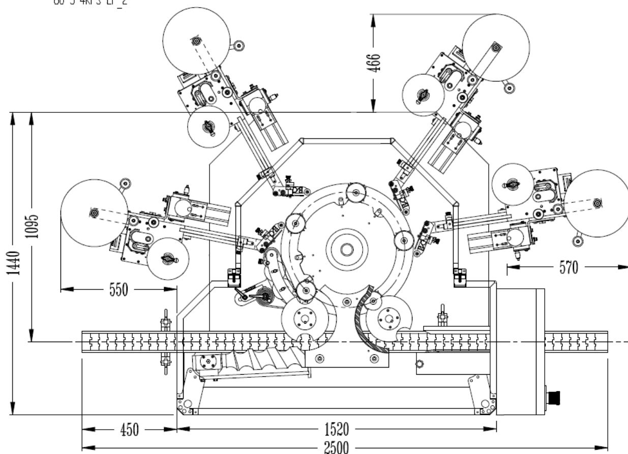
G CAVAGNINO & GATTI Spa MODELLO CG 80-5-4RPS-CF 80-5-4RPS-CF_2
